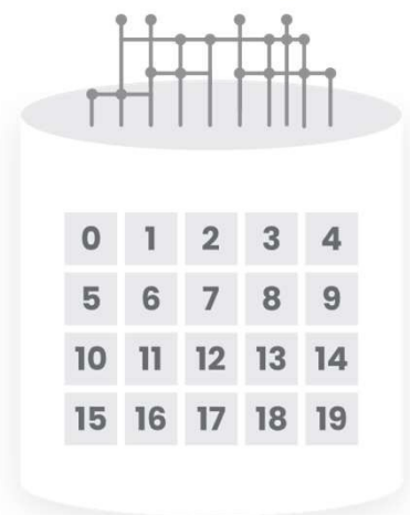
File Storage
