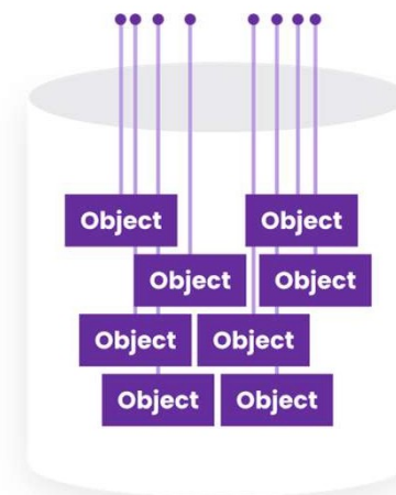
Object Storage
